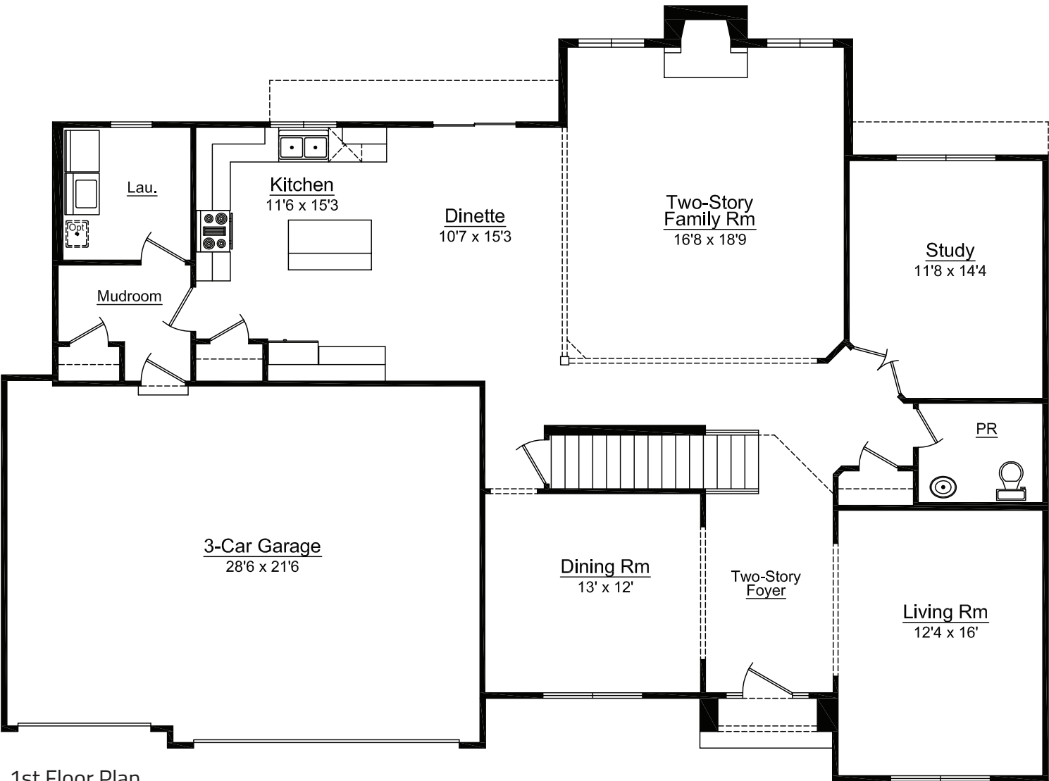
1st Floor Plan 1,732 sq. ft.
